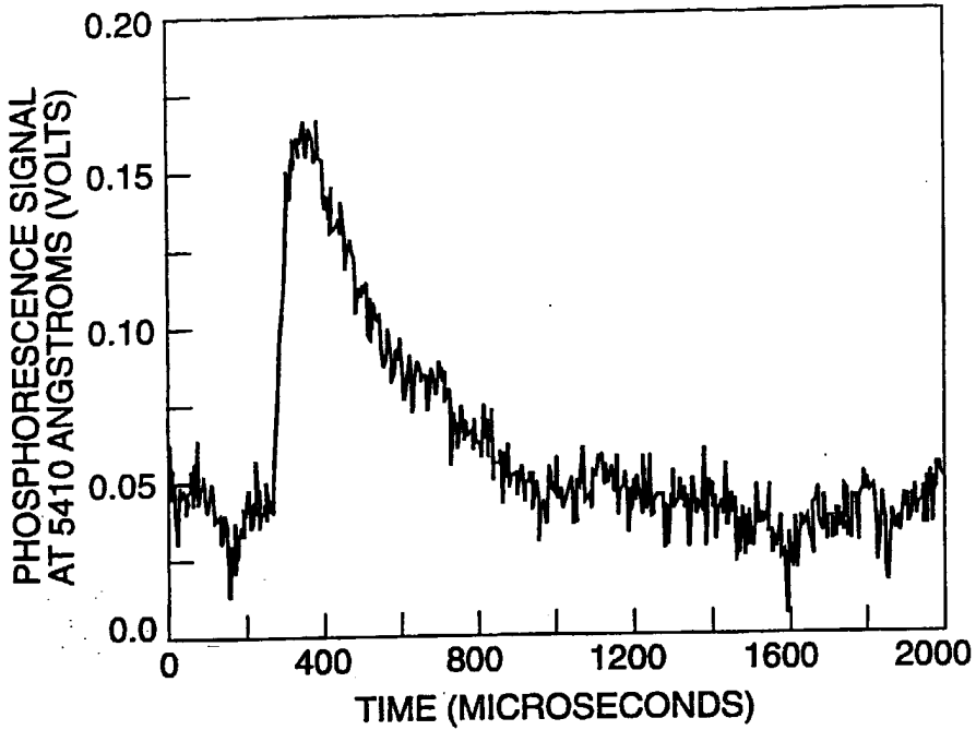
TIME DECAY OF REPORTER PHOSPHORESCENCE
